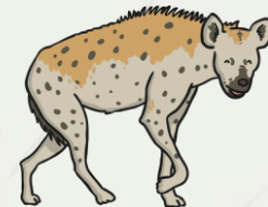
hyena
